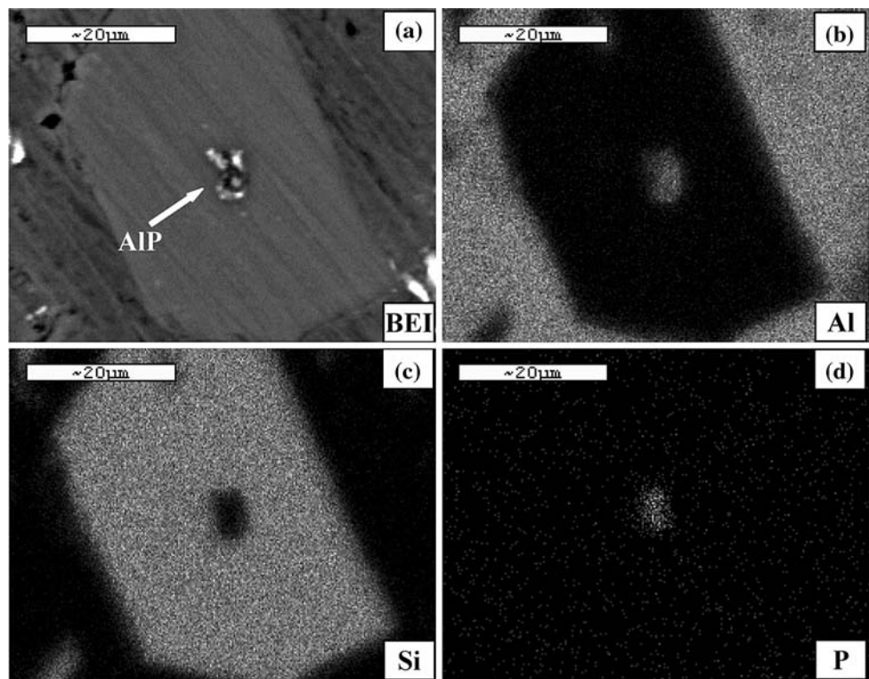
Fig. 7 EPMA analysis of A390 alloys with addition of Al–17Si–2.5P master alloys: a BEI and b–d the X-ray images for element: Al, Si, and P, respectively
