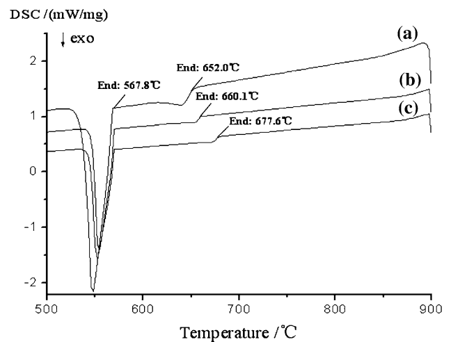
Fig. 8 DSC results for Al–18Si alloys: a without Al–Si–P addition, b Al–18Si + 1.5% Al–17Si–2.5P (Test No.8: A3–B2–C1), c Al–18Si + 1.5% Al–17Si–2.5P (treated with the predicted optimal processing parameters: A3–B3–C1)
